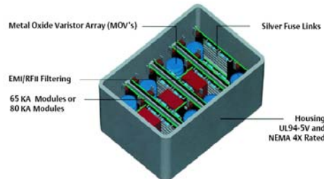
Liebert 510 Series - ACCUVAR Category Type 1 - Service Entrance Rated
